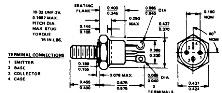
TO-111 (ISOLATED)
