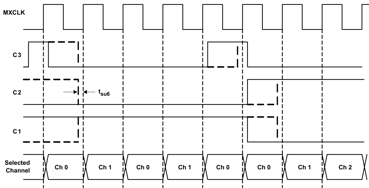
Figure 7. Multiplexer Auto Mode Timing Diagram
