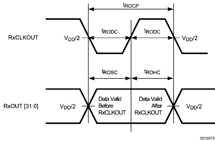
FIGURE 9. Deserializer Setup and Hold times
