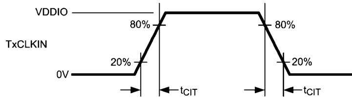
FIGURE 4. Serializer Input Clock Transition Time
