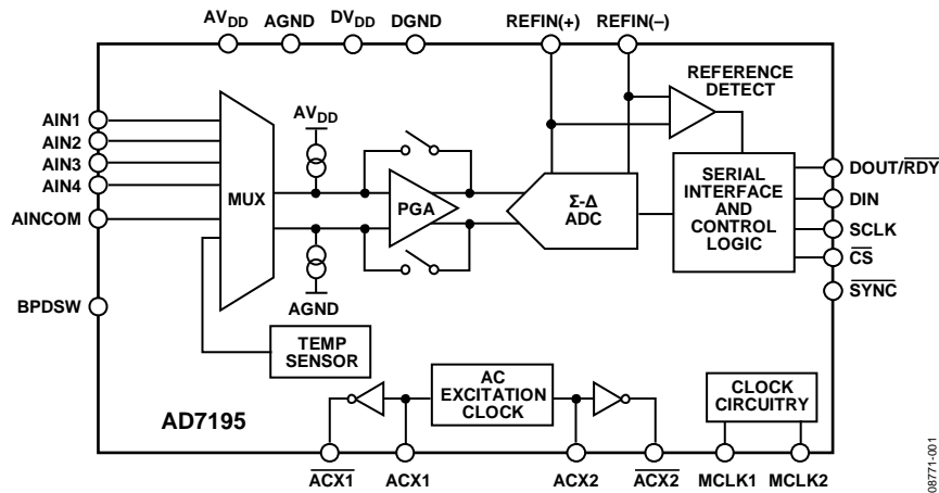
Figure 18. Block Diagram
