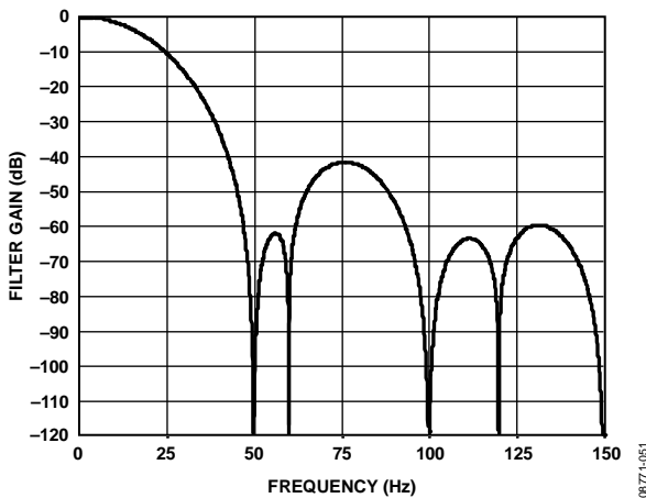
Figure 39. Sinc 3 Filter Response (FS[9:0] = 96, REJ60 = 1)
