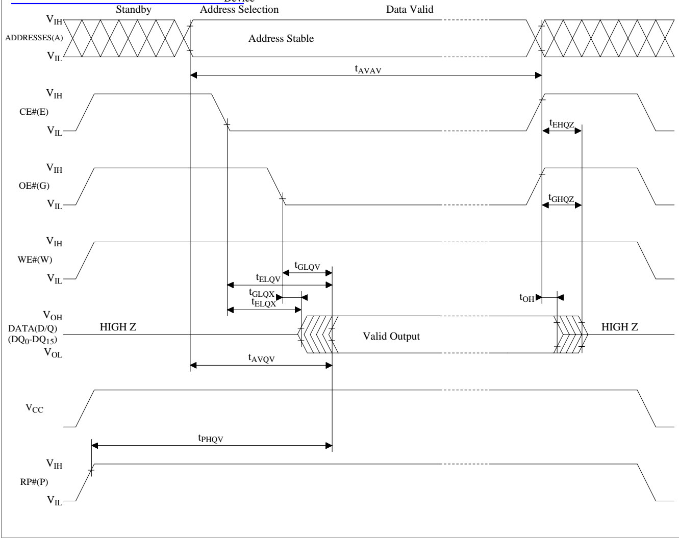
Figure 14. AC Waveform for Read Operations
