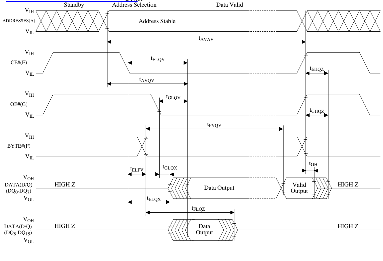
Figure 15. BYTE# timing Waveform
