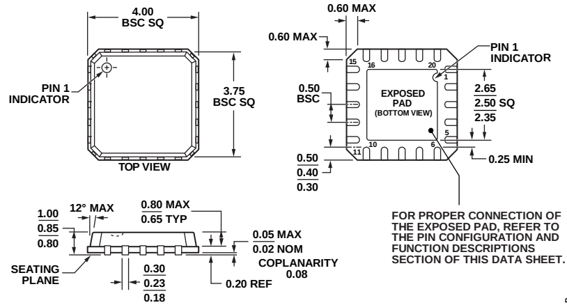
COMPLIANT TO JEDEC STANDARDS MO-220-VGGD-1 Figure 30. 20-Lead Lead Frame Chip Scale Package [LFCSP_VQ] 4 mm x 4 mm Body, Very Thin Quad (CP-20-4) Dimensions shown in millimeters
