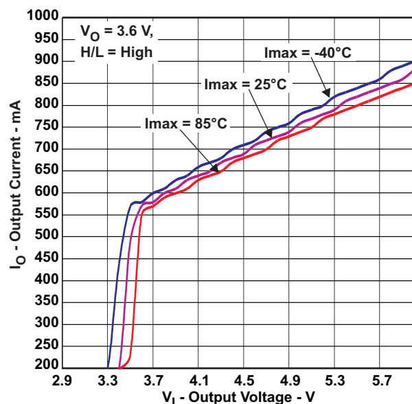
Figure 1. Maximum Output Current
