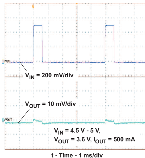
Figure 20. Line Transient
