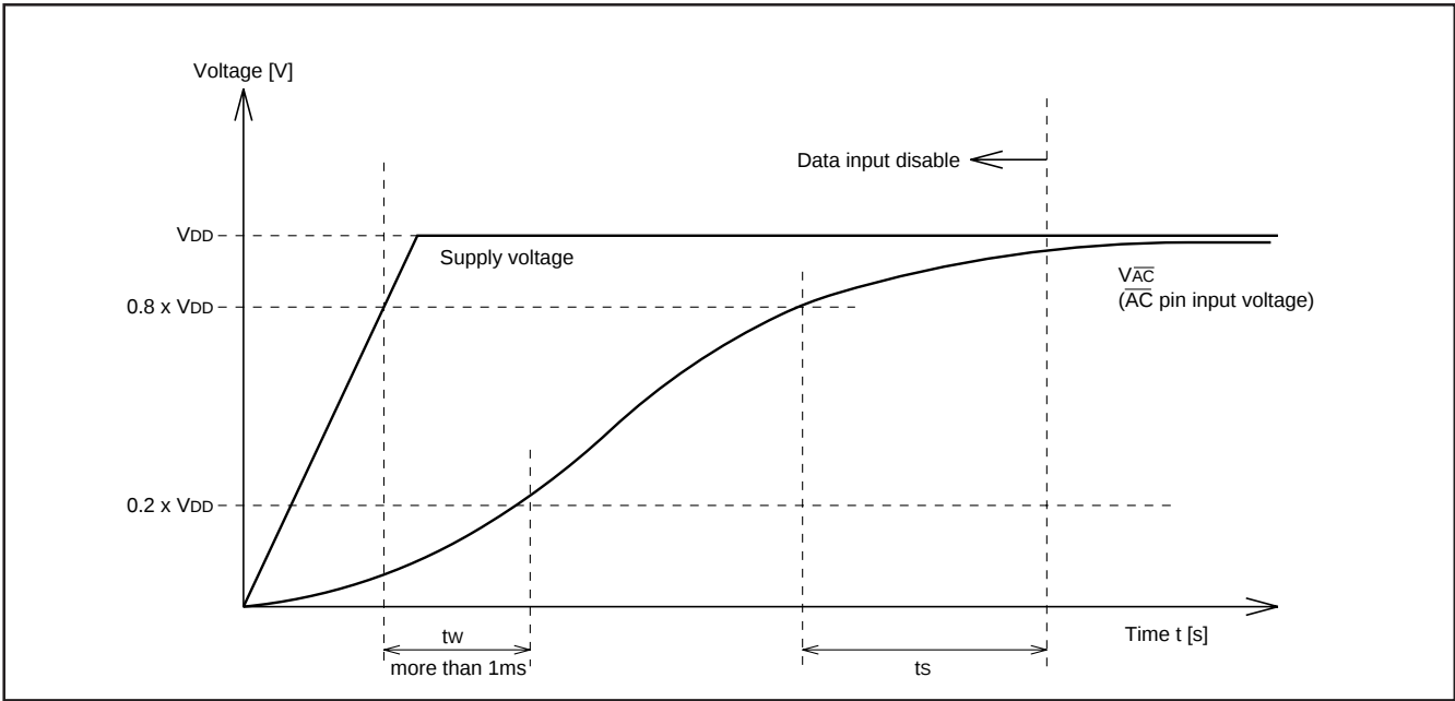
Fig.26 Timing of power supplying to \overline{AC} pin
