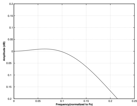
Figure 39. Quad-Speed (fast) Passband Ripple
