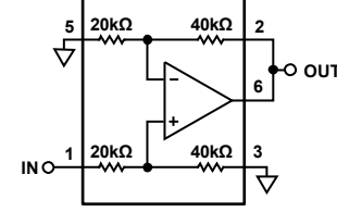
Figure 54. Noninverting Amplifier, Gain = 2
