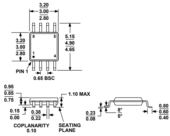
COMPLIANT TO JEDEC STANDARDS MO-187-AA Figure 58. 8-Lead Mini Small Outline Package [MSOP] (RM-8) Dimensions shown in millimeters
