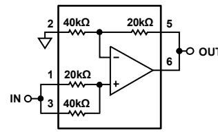
Figure 53. Noninverting Amplifier, Gain = 1.5
