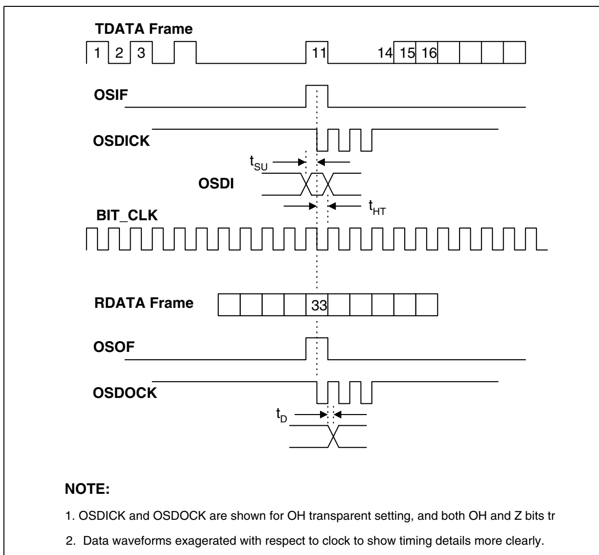
Figure 16. OSIO Timing
