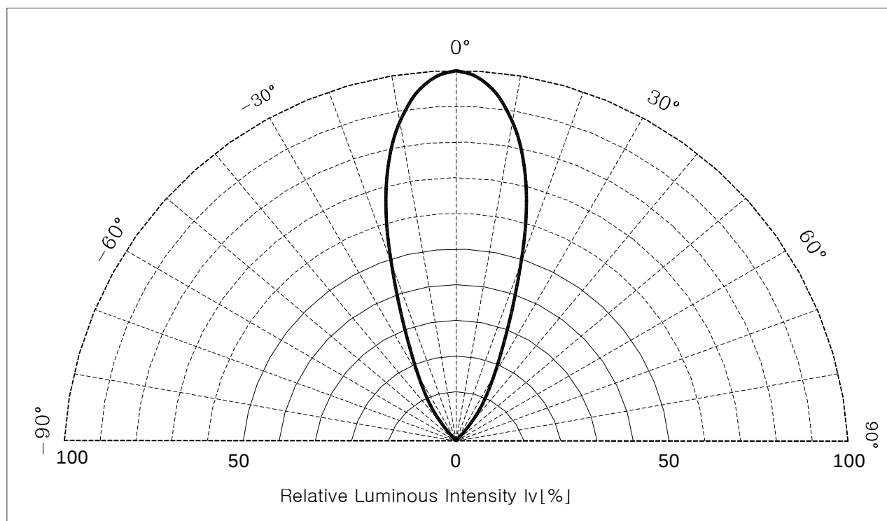
Fig. 6 Radiation Diagram
