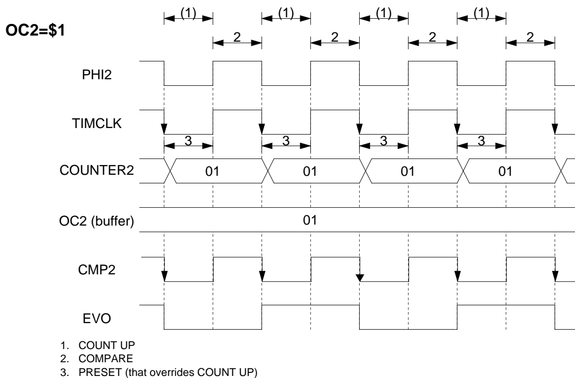
Figure 8-5: Timer 2 Timing for f(\text{PHI2}) = f(\text{TIMCLK})
