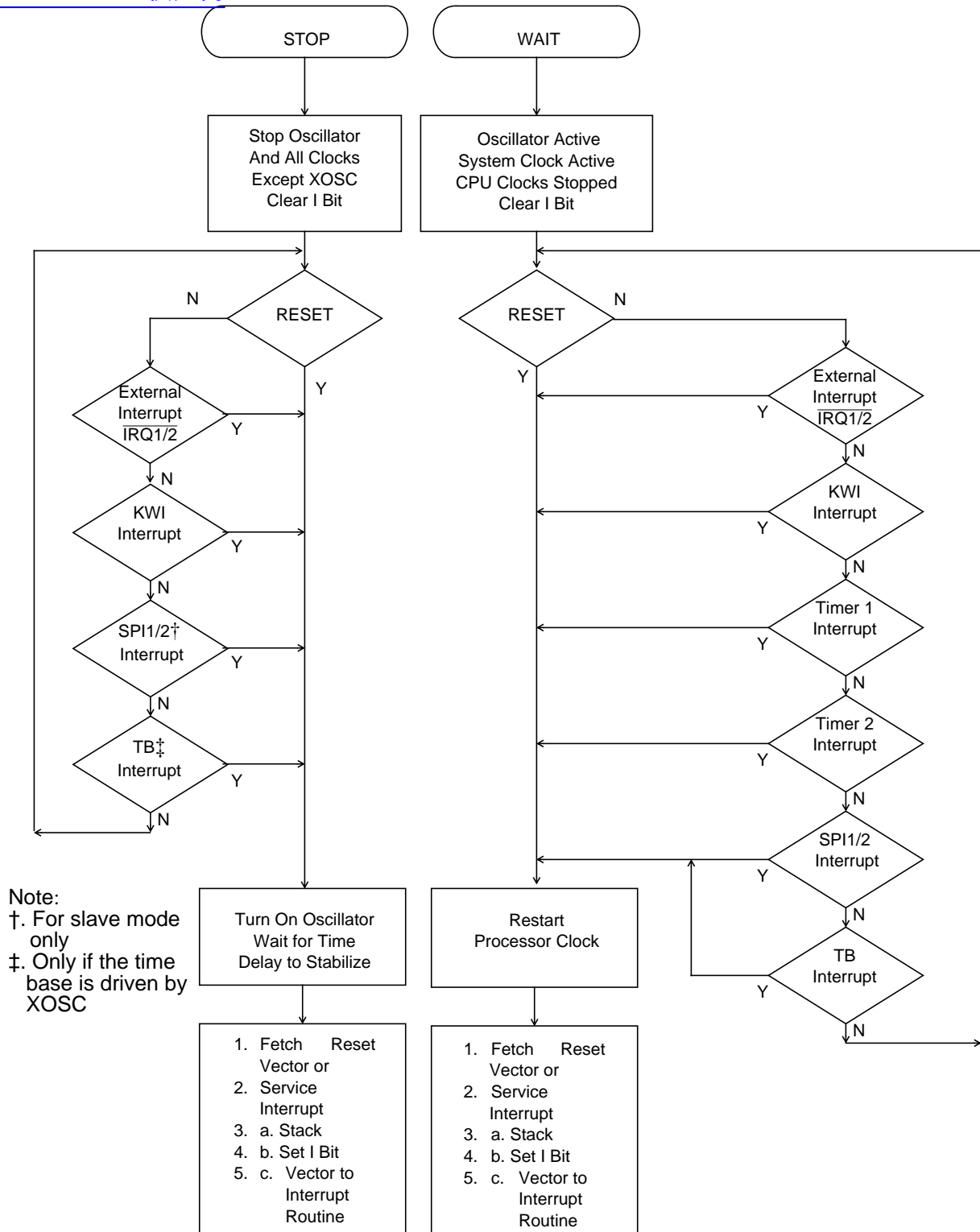
Figure 4-3: STOP/WAIT Flowcharts
