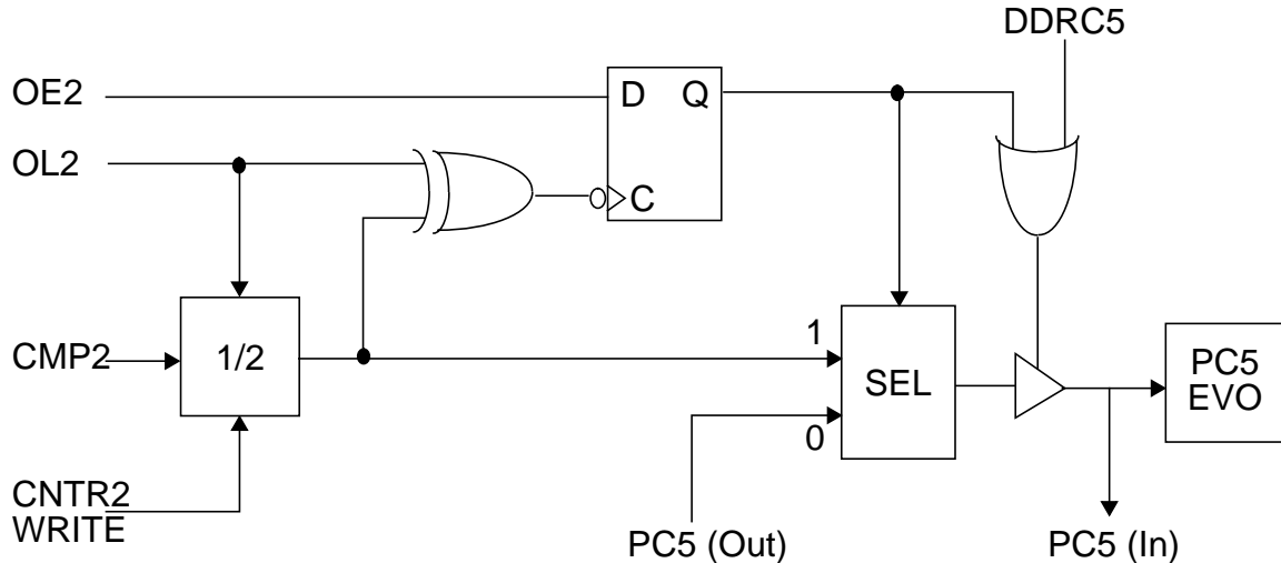
Figure 8-9: EVO Block Diagram
