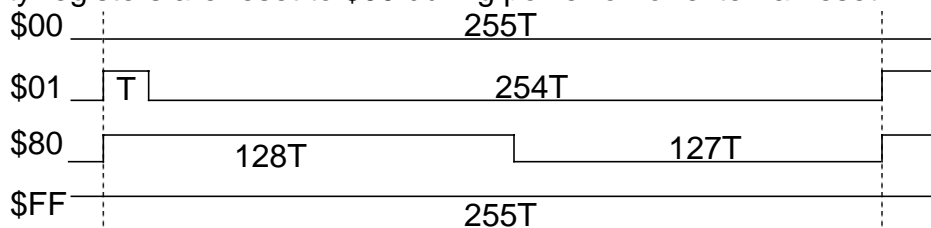
Figure 9-4: PWM Waveform Examples (E = 2MHz; CLK = E/2)
