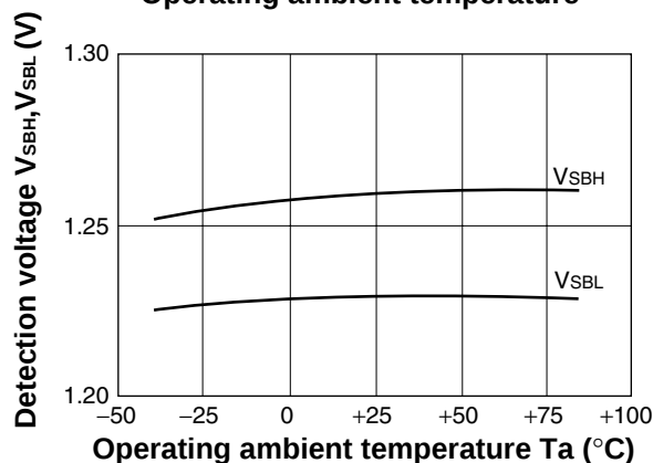
Detection voltage ( V_{SB} ) vs. Operating ambient temperature
