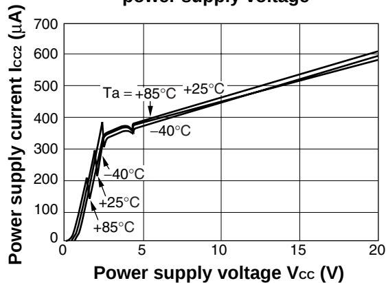
Power supply current ( I_{CC2} ) vs. power supply voltage
