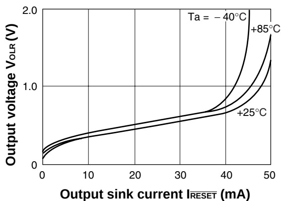
Output voltage ( V_{OLR} ) vs. output sink current
