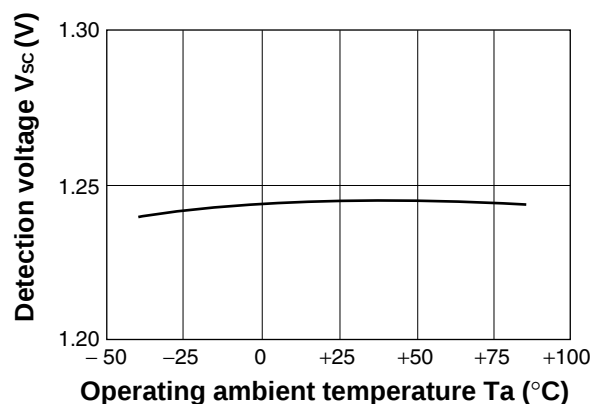
Detection voltage ( V_{SC} ) vs. Operating ambient temperature
