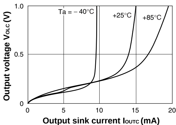
Output voltage ( V_{OLC} ) vs. output sink current
