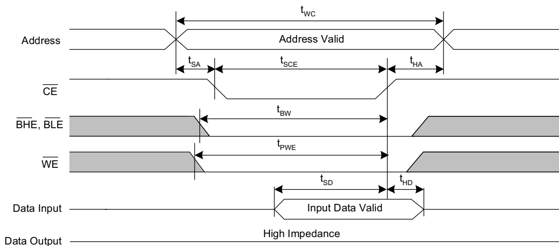
Figure 10. SRAM Write Cycle #2: \overline{\text{CE}} Controlled [3, 22, 23, 24]
