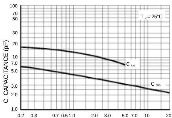
Figure 7. Capacitances Figure
