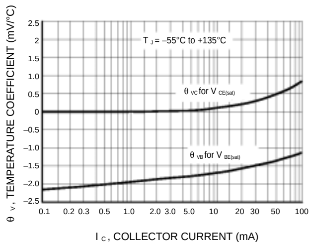
Figure 5. Temperature Coefficients
