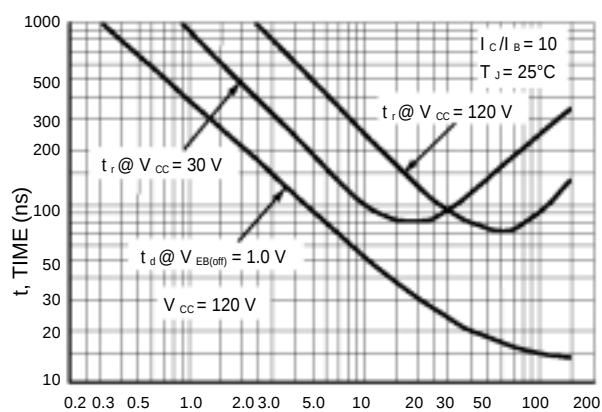
8. Turn-On Time
