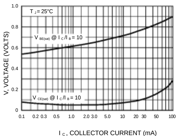
Figure 4. "On" Voltages
