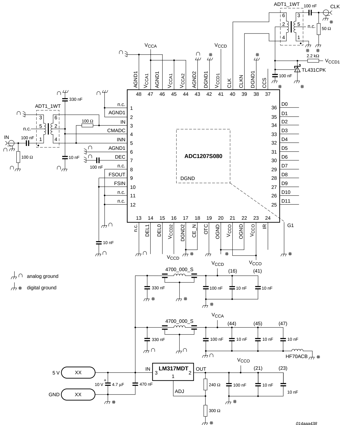
Fig 10. Application diagram
