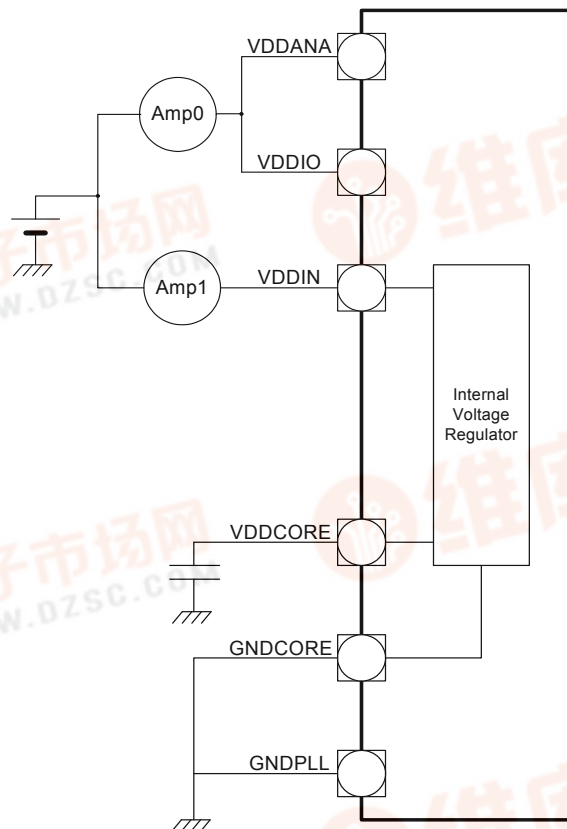
Figure 10-4. Measurement Setup
