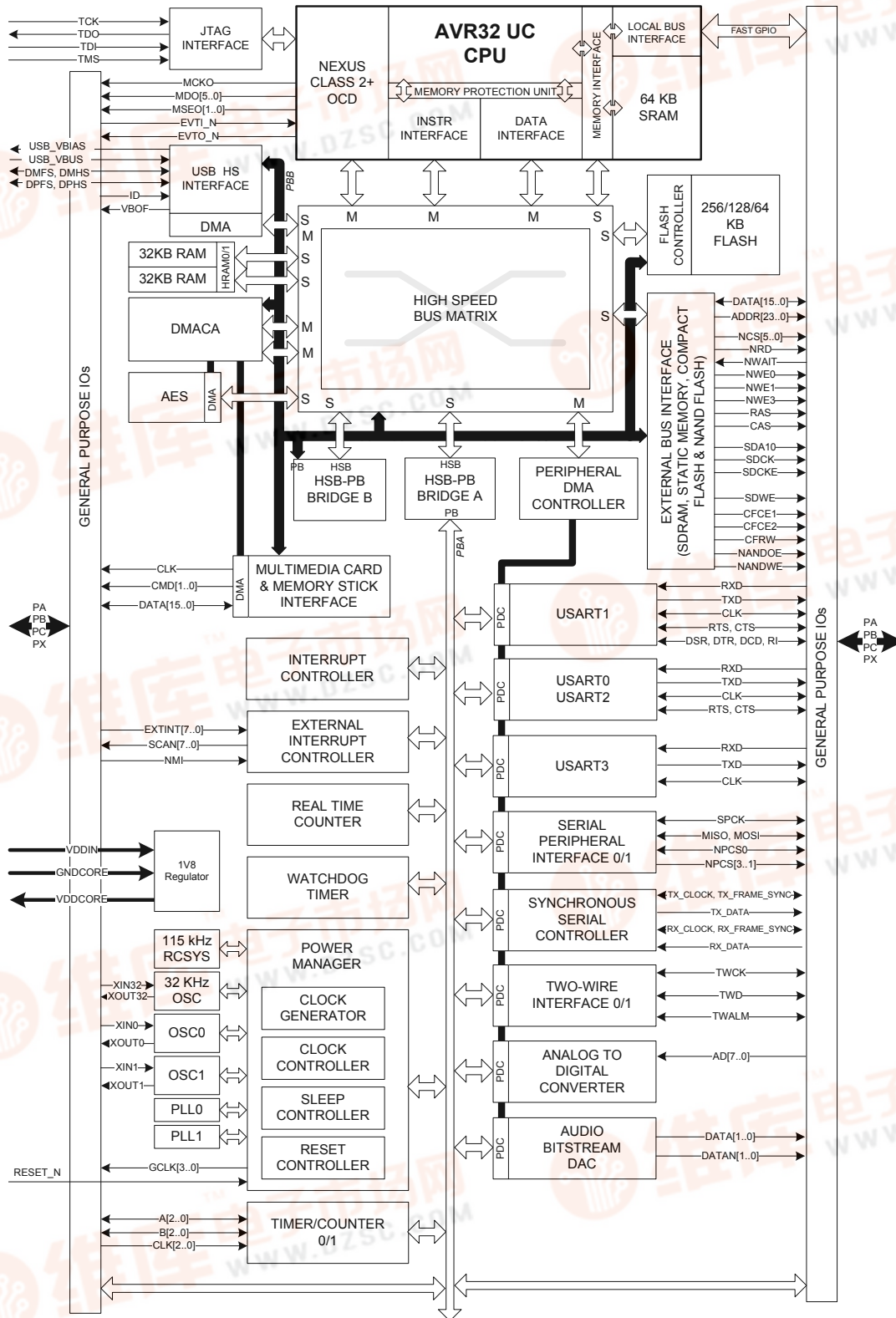
Figure 2-1. Blockdiagram
