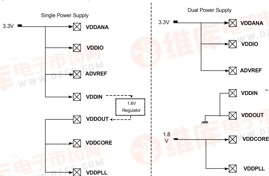
Figure 5-1. Power Supply
