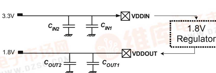
Figure 5-2. Supply Decoupling
