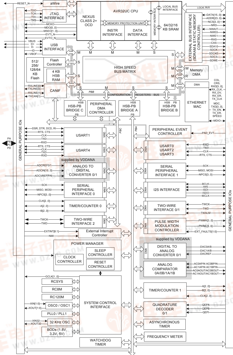
Figure 2-1. Block diagram
