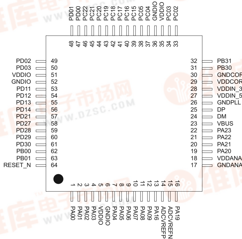
Figure 3-1. QFN64/TQFP64 Pinout
