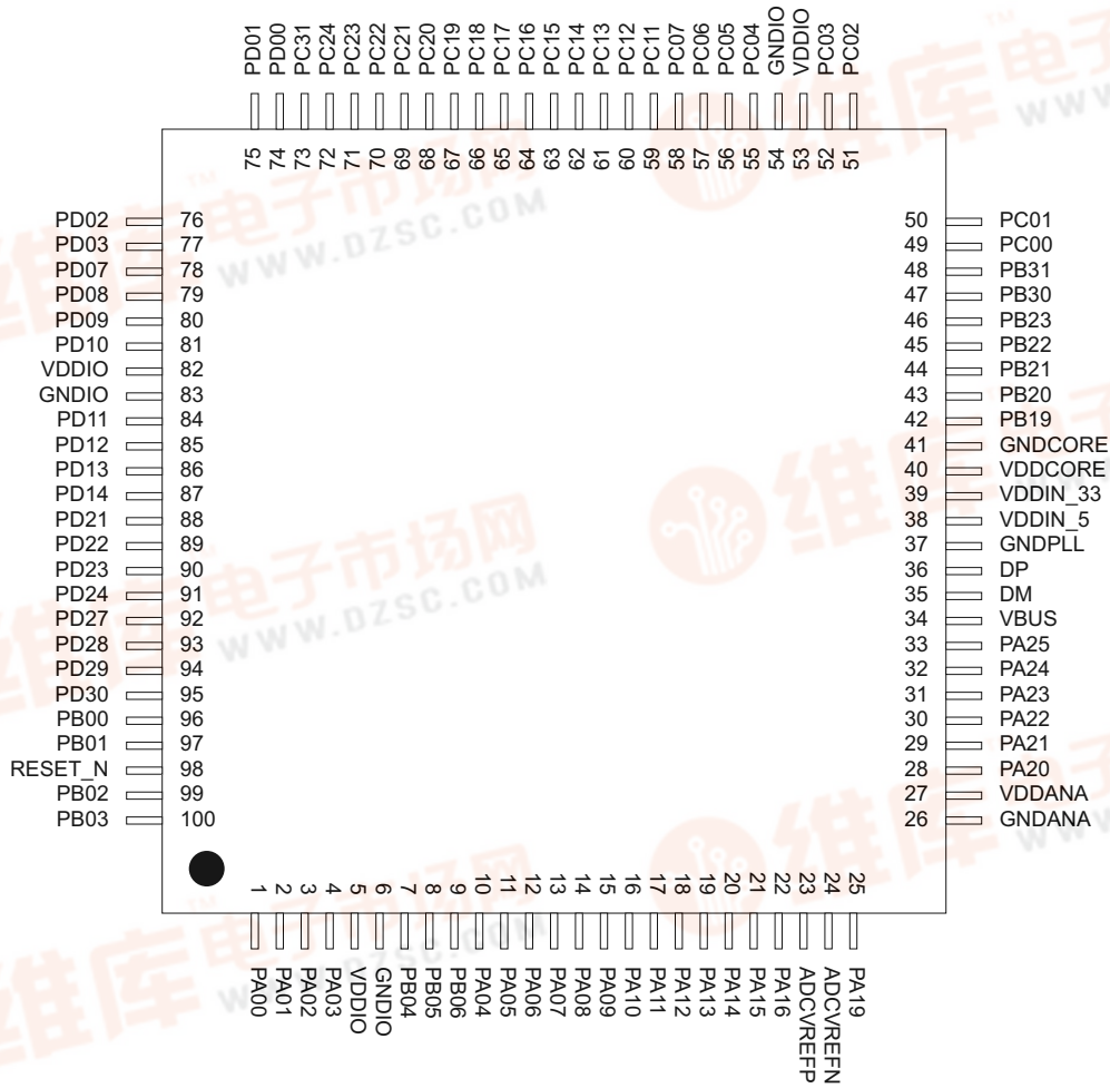
Figure 3-2. TQFP100 Pinout
