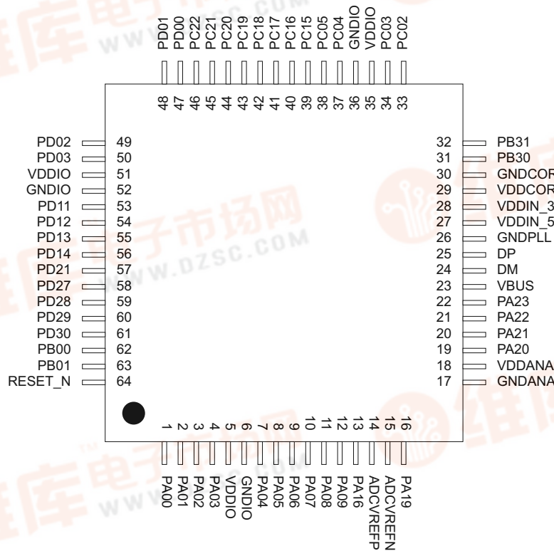
Figure 3-1. QFN64/TQFP64 Pinout
