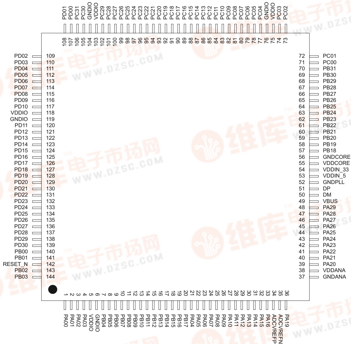
Figure 3-3. LQFP144 Pinout
