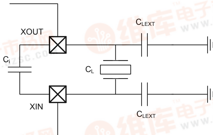
Figure 7-2. Oscillator Connection
