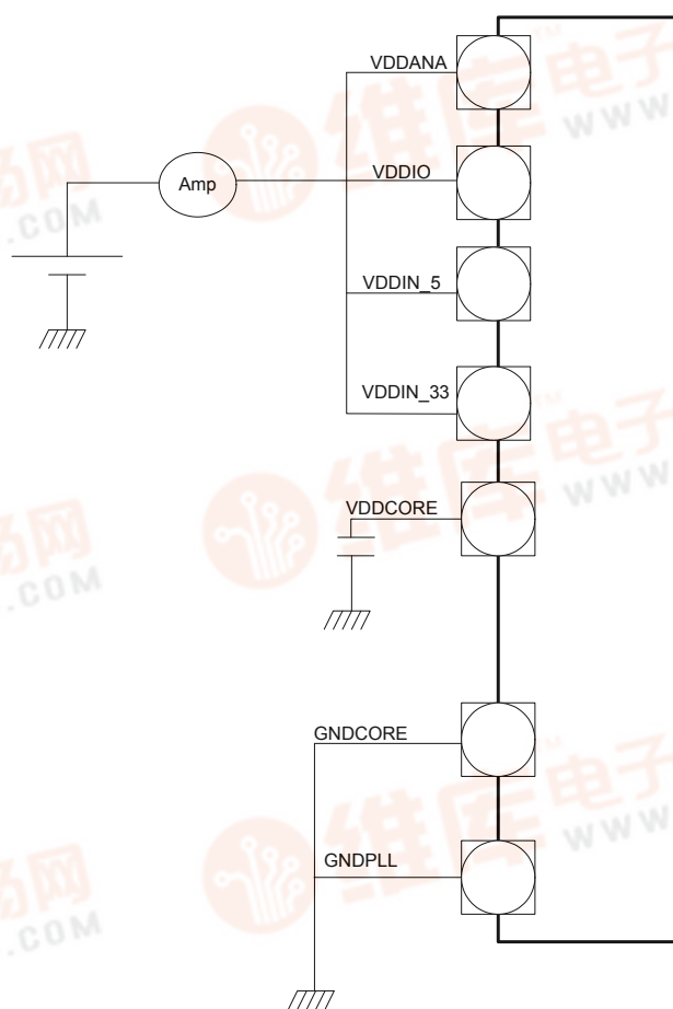
Figure 7-1. Measurement Schematic
