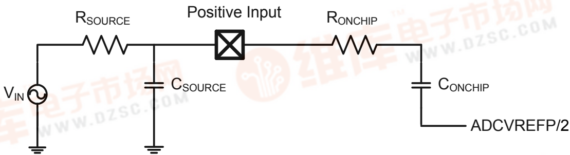
Figure 7-7. ADC Input
