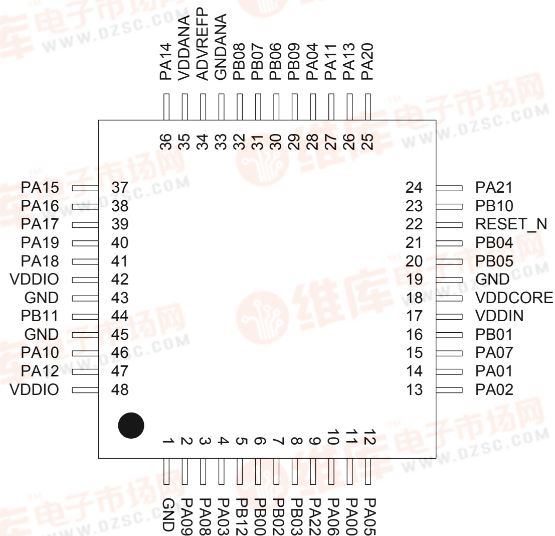
Figure 3-1. TQFP48/QFN48 Pinout
