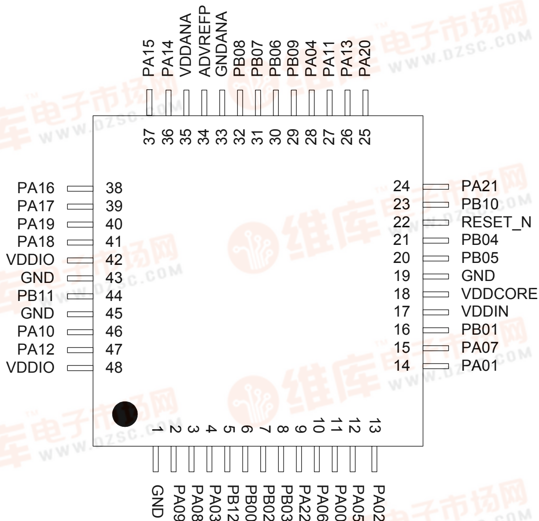
Figure 3-2. TLLGA48 Pinout
