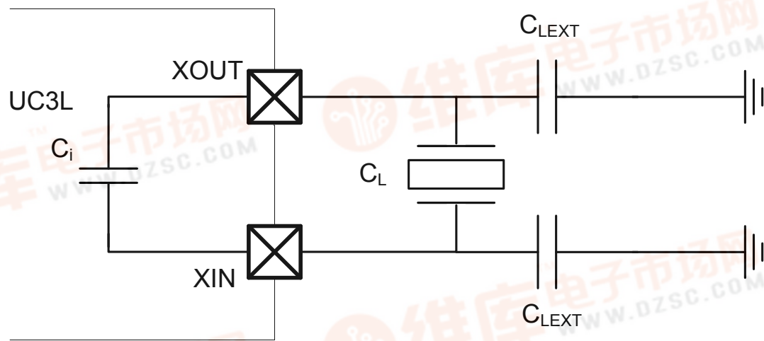
Figure 7-3. Oscillator Connection
