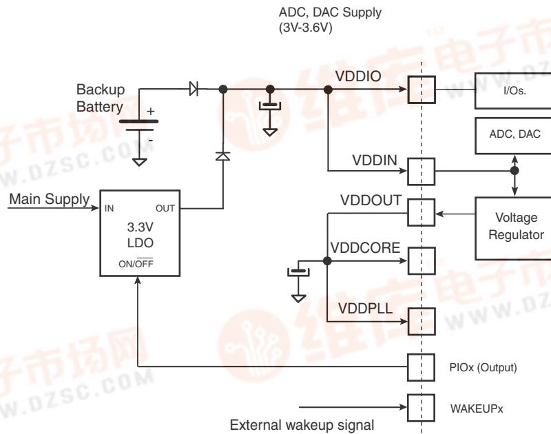
Figure 5-3. Core Externally Supplied (backup battery)
