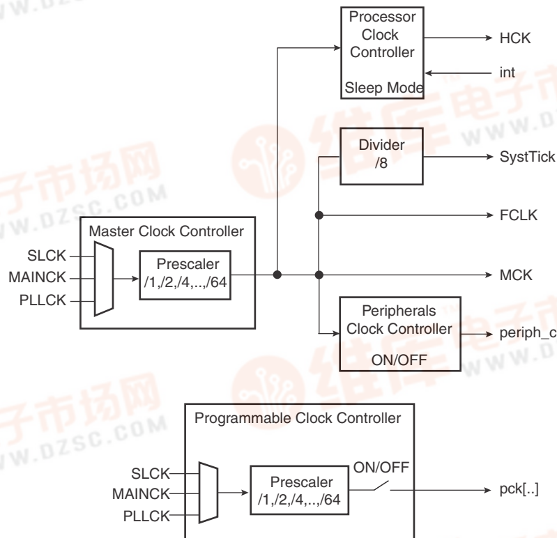
Figure 9-3. SAM3N4/2/1 Power Management Controller Block Diagram
