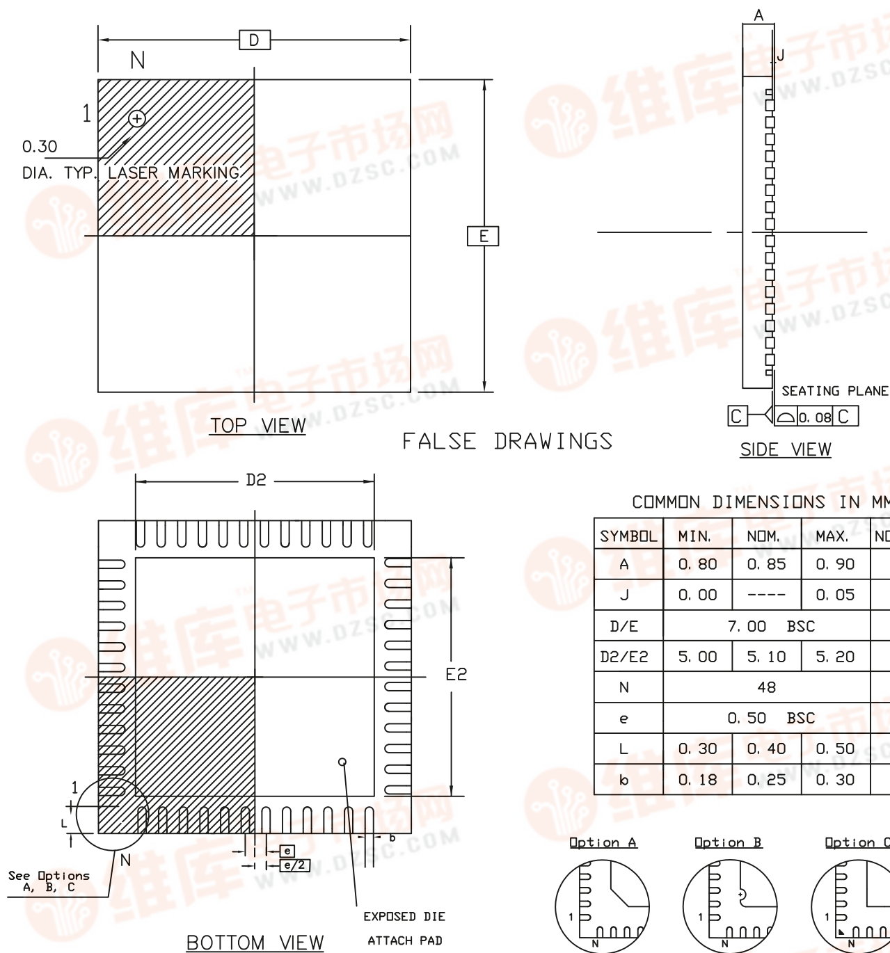
Figure 12-4. 48-pad QFN Package Drawing
