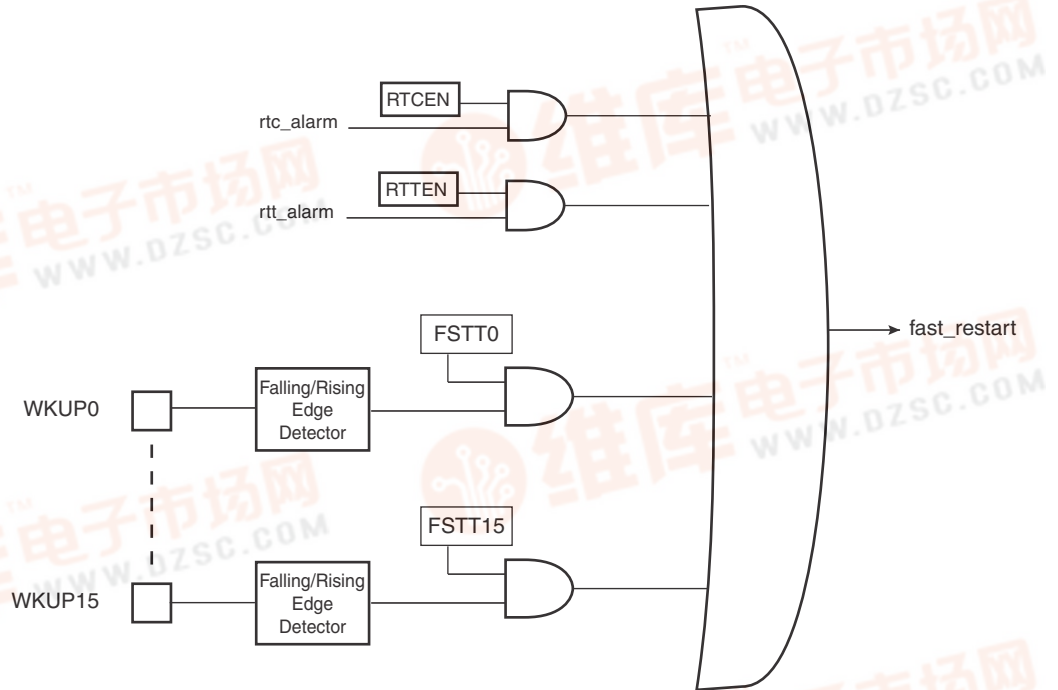
Figure 5-5. Fast Start-Up Sources
