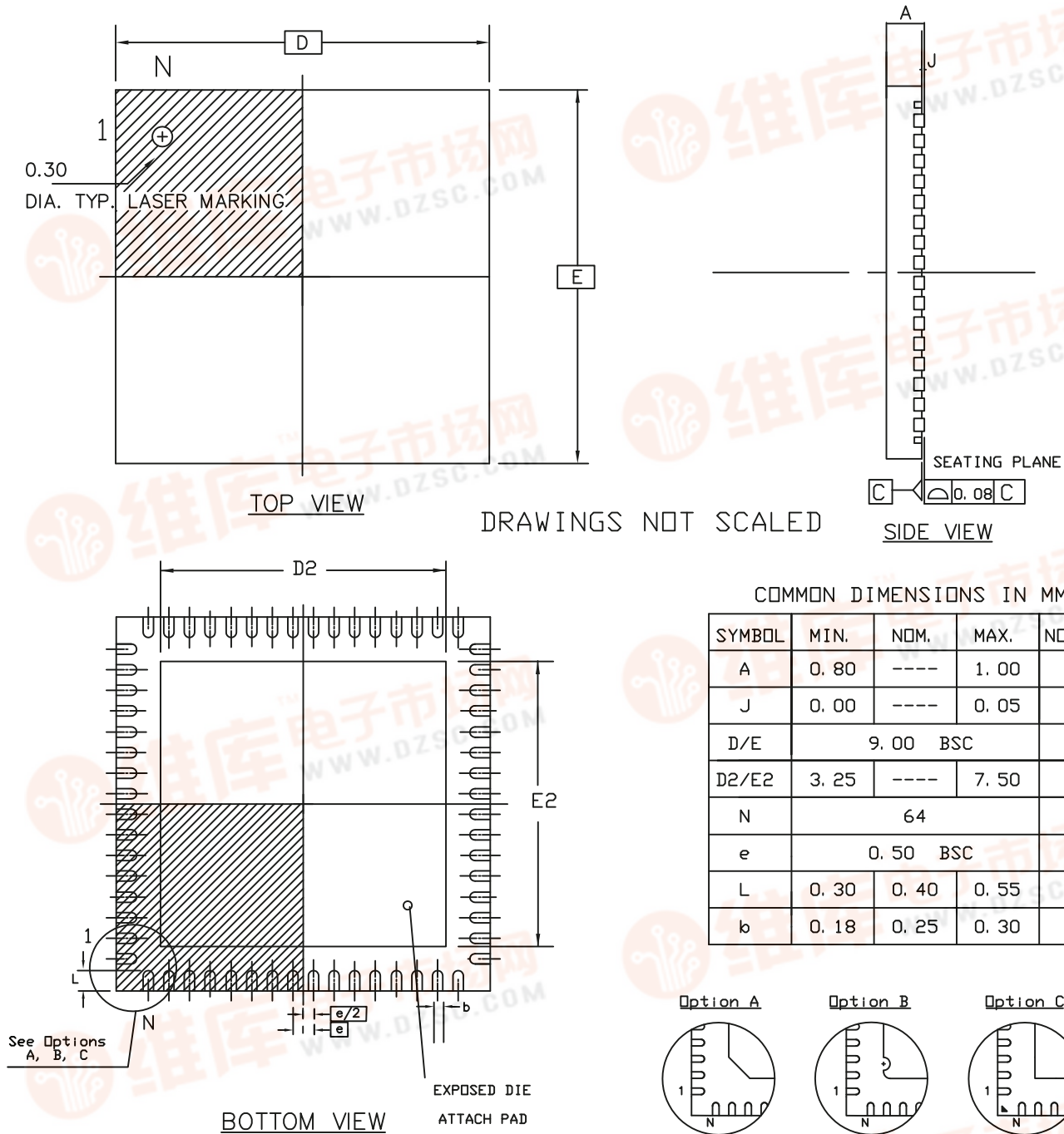
Figure 12-5. 64-pad QFN Package Drawing
