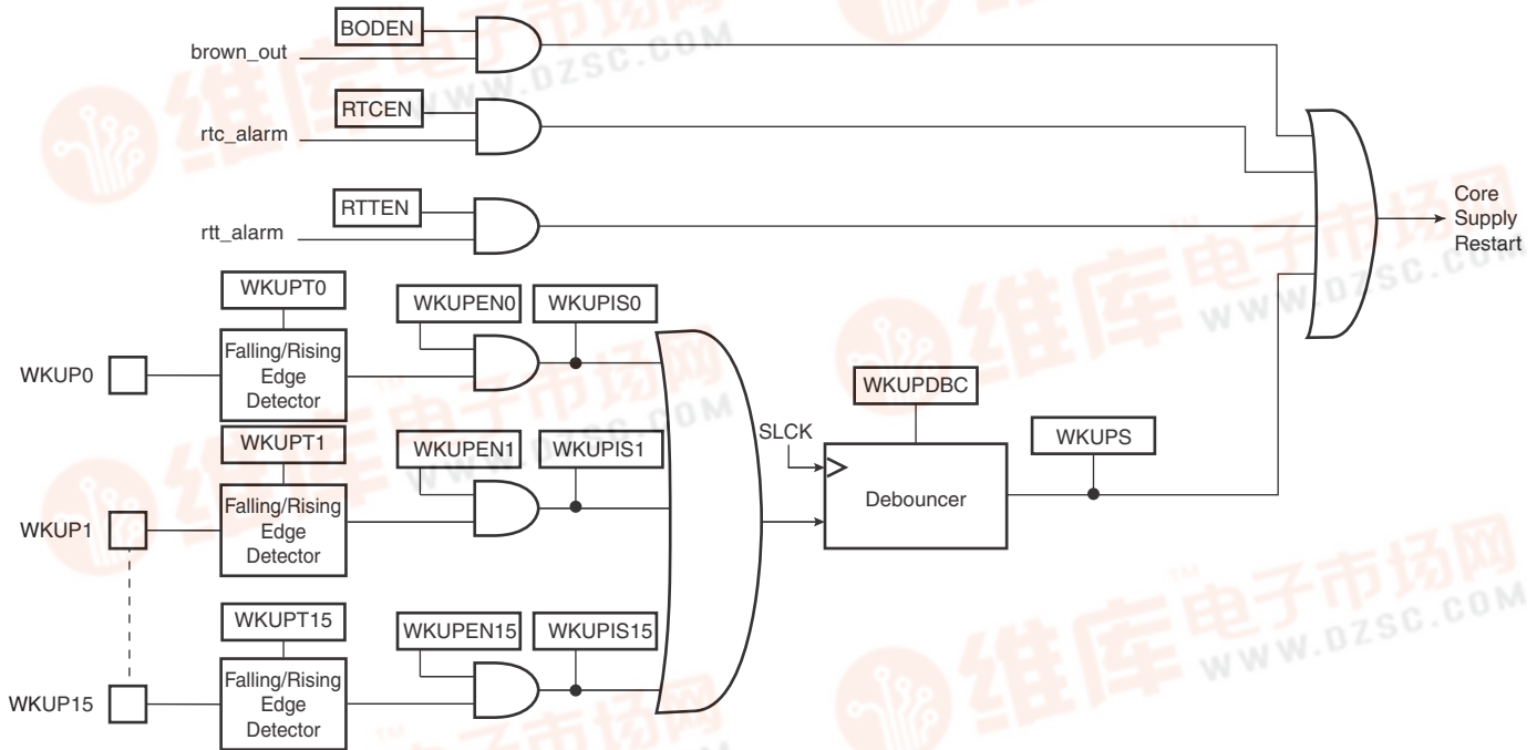
Figure 5-4. Wake-up Source
