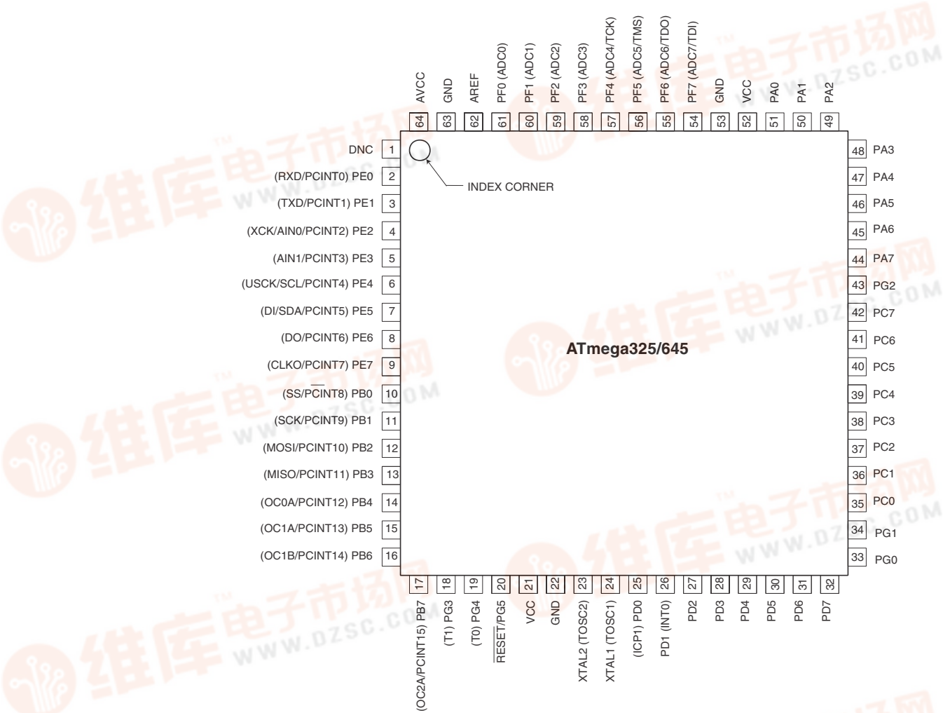
Figure 1-2. Pinout ATmega325/645
