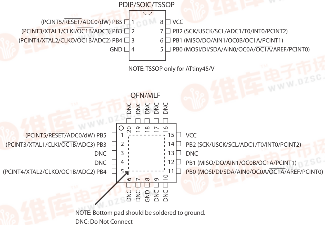
Figure 1-1. Pinout ATtiny25/45/85
