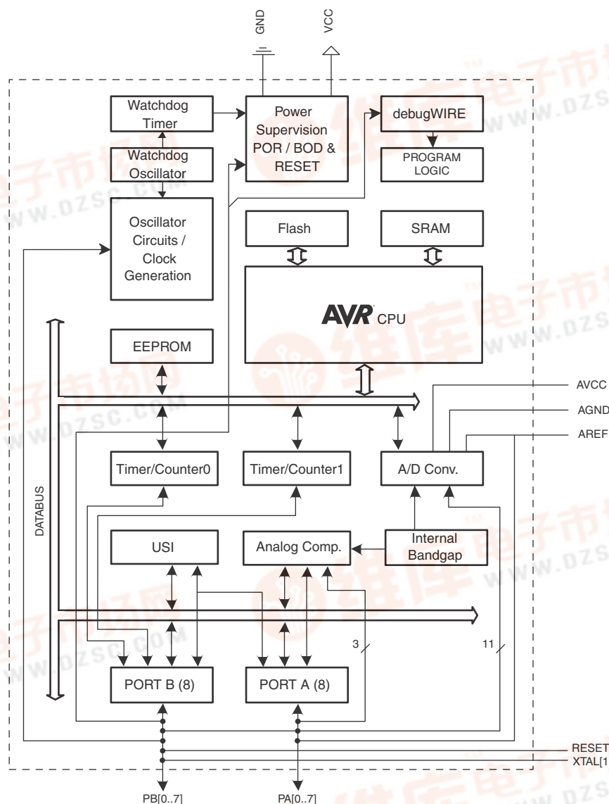
Figure 2-1. Block Diagram
