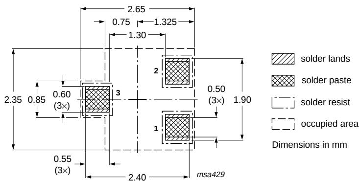
Fig 18. Reflow soldering footprint BAW56W (SOT323/SC-70)
