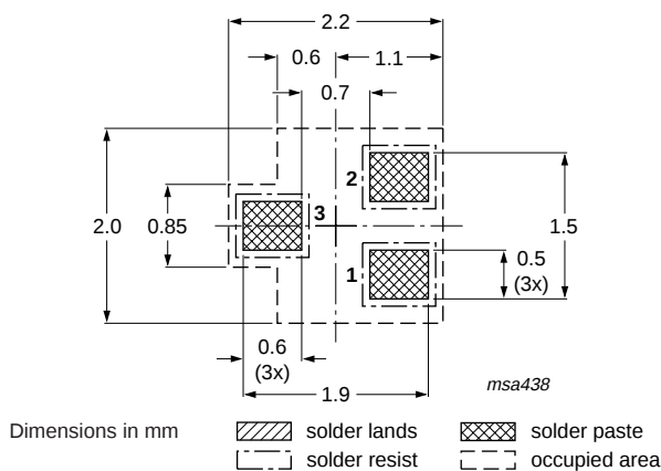
Fig 17. Reflow soldering footprint BAW56T (SOT416/SC-75)
