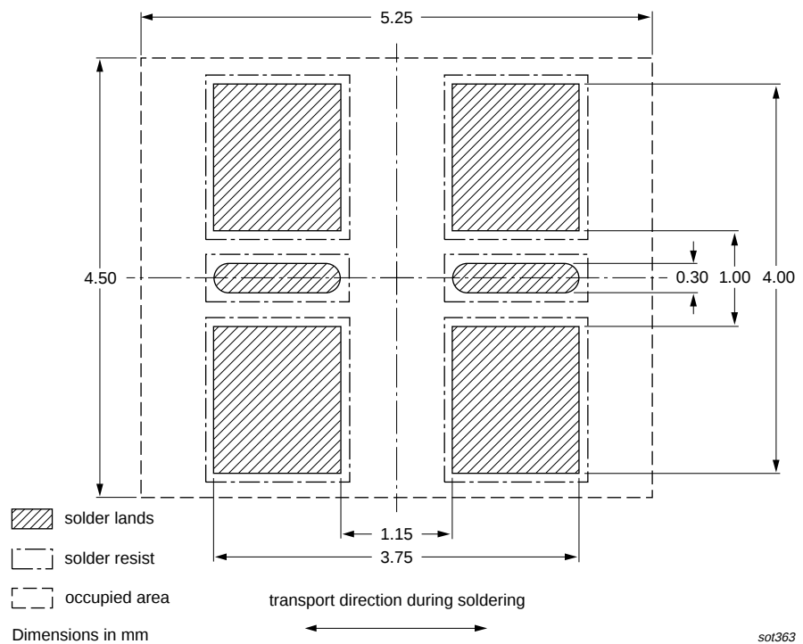
Fig 16. Wave soldering footprint BAV756S and BAW56S (SOT363/SC-88)
