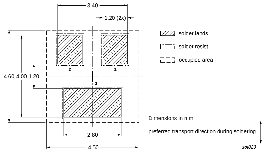
Fig 13. Wave soldering footprint BAW56 (SOT23/TO-236AB)
