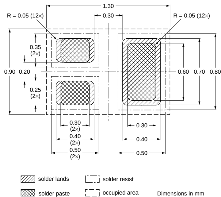
Fig 14. Reflow soldering footprint BAW56M (SOT883/SC-101)
