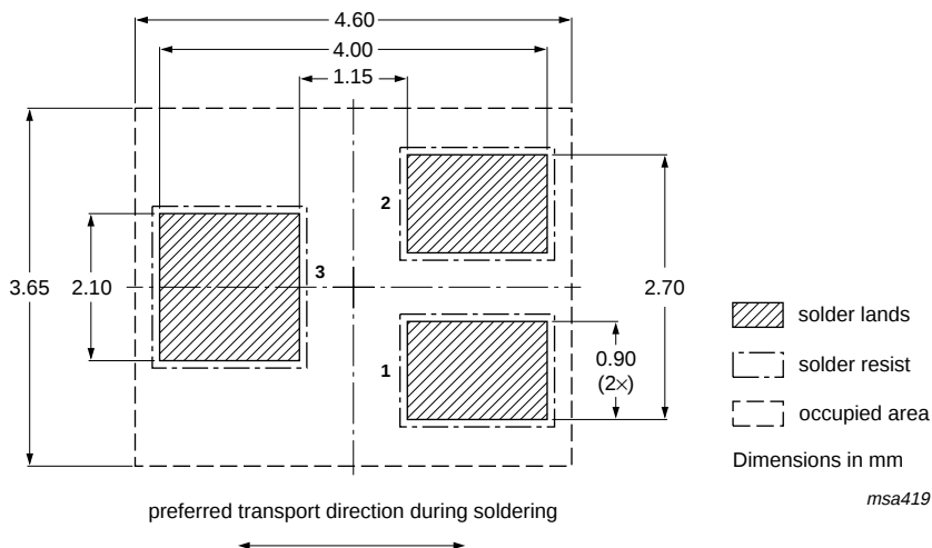
Fig 19. Wave soldering footprint BAW56W (SOT323/SC-70)
