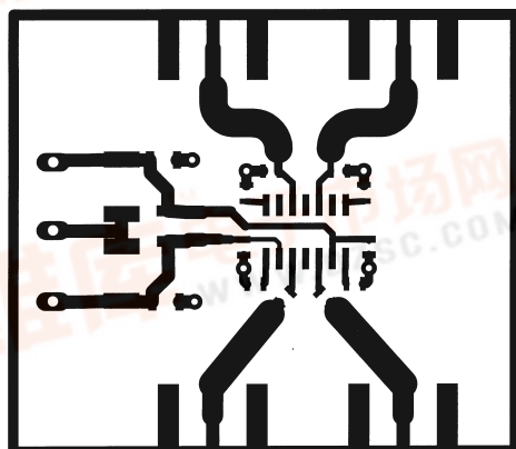
Top Silk
