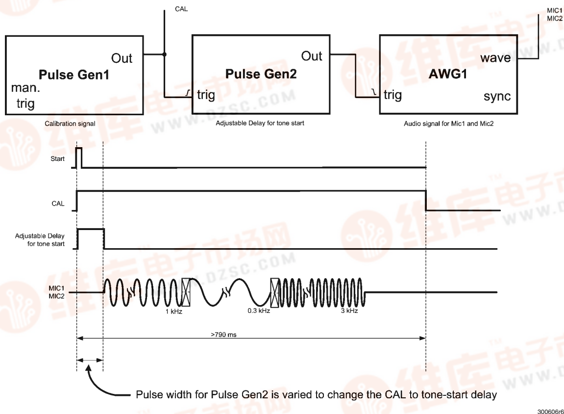
FIGURE 19. Example of Three Tone Signal Generation
