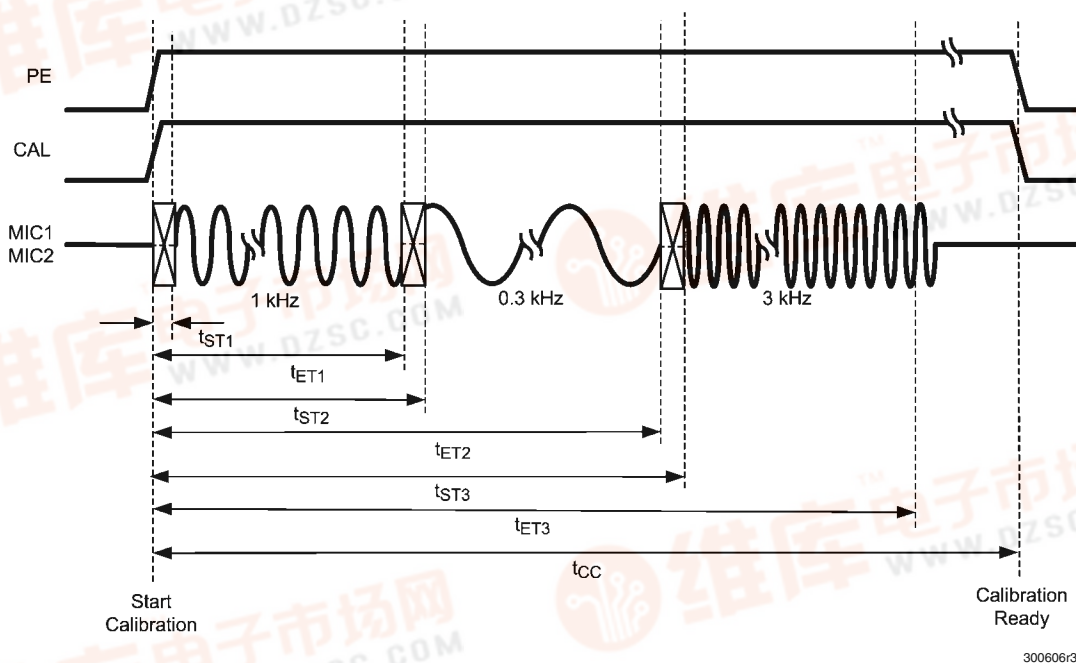
FIGURE 18. Calibration Timing
