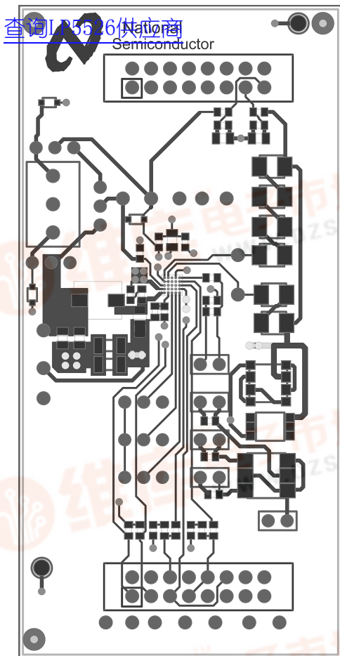
Fig. 12 Lp5526 Evaluation Board Layer 1 (Top, Signal).
