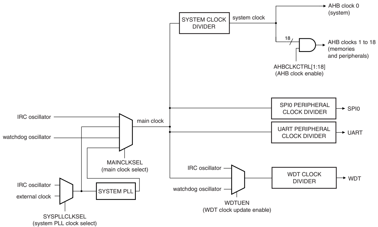
Fig 4. LPC1102 clock generation block diagram
