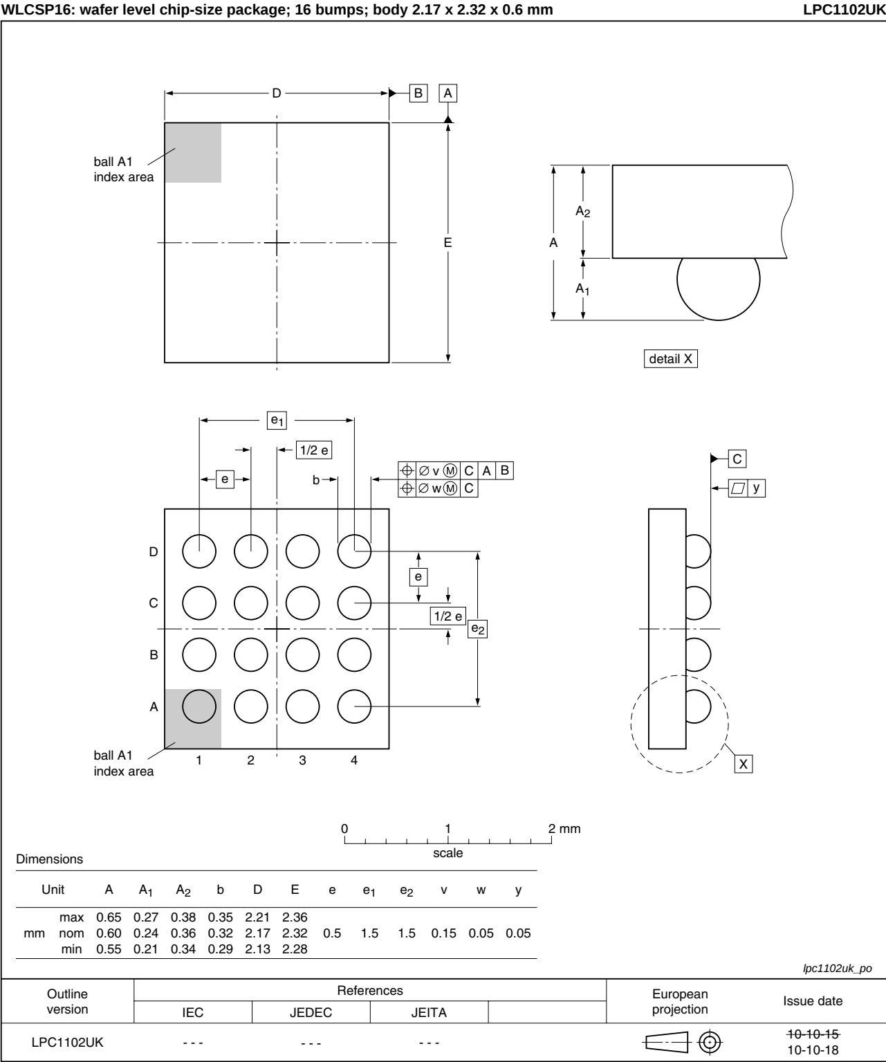
Fig 21. Package outline (WLCSP16)
