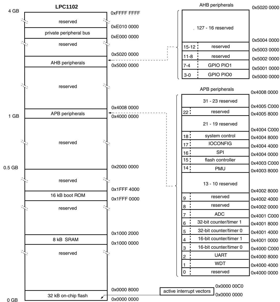
Fig 3. LPC1102 memory map
