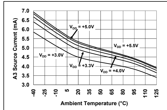
FIGURE 2-22: Amplifier A3 Source Current vs. Temperature.
