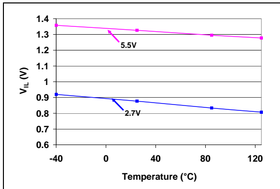
FIGURE 2-52: V_{IL} (SDI, SCK, \overline{\text{CS}} , \overline{\text{WP}} , and SHDN) vs. V_{DD} and Temperature.
