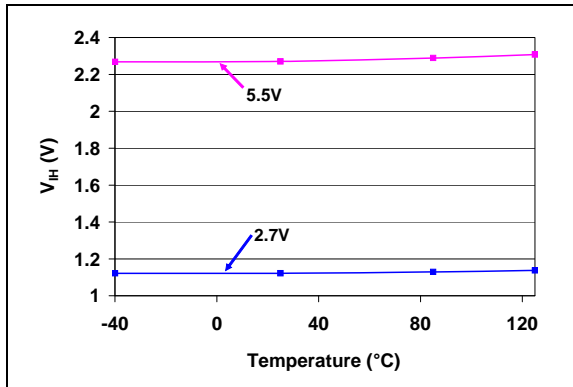
FIGURE 2-51: V_{IH} (SDI, SCK, \overline{\text{CS}} , \overline{\text{WP}} , and SHDN) vs. V_{DD} and Temperature.
