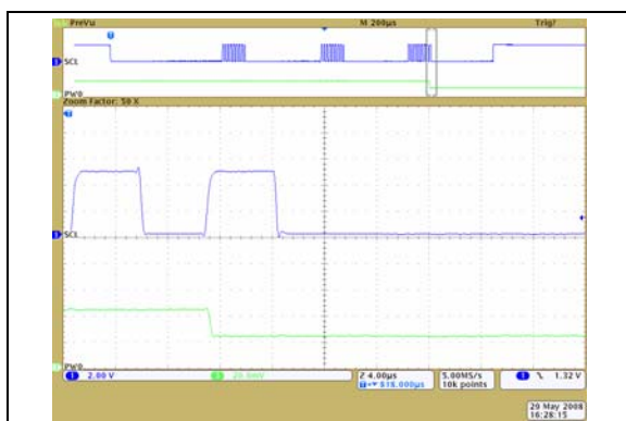
FIGURE 2-28: 10 k \Omega – Low-Voltage Decrement Wiper Settling Time ( V_{DD} = 2.7V ) (1 \mu s/Div ).
