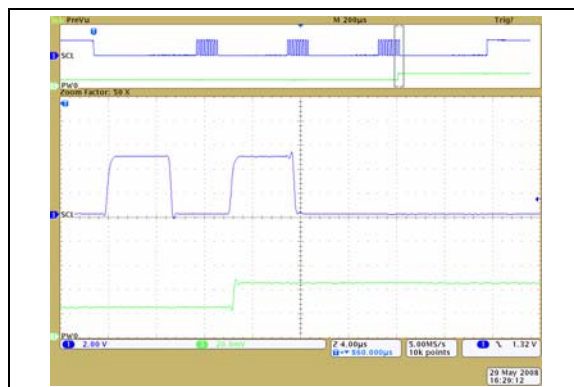
FIGURE 2-30: 10 k \Omega – Low-Voltage Increment Wiper Settling Time ( V_{DD} = 5.5V ) (1 \mu s/Div ).
