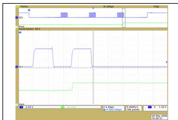
FIGURE 2-31: 10 k \Omega – Low-Voltage Increment Wiper Settling Time ( V_{DD} = 2.7V ) (1 \mu s/Div ).
