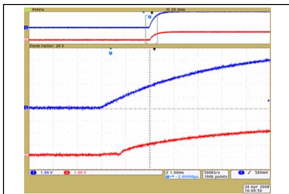
FIGURE 2-29: 10 k \Omega – Power-Up Wiper Response Time (1 \mu s/Div).
