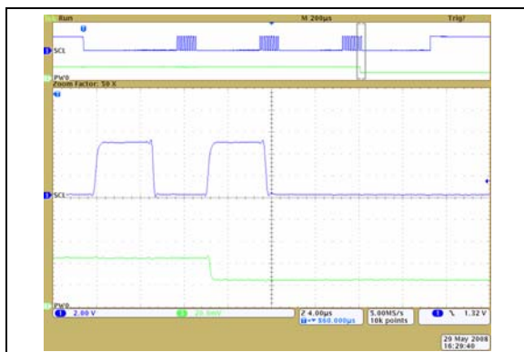
FIGURE 2-27: 10 k \Omega – Low-Voltage Decrement Wiper Settling Time ( V_{DD} = 5.5V ) (1 \mu s/Div ).
