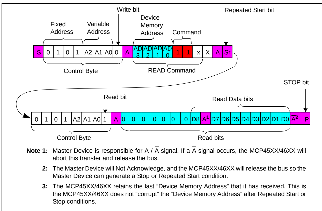
FIGURE 7-5: I 2 C Random Read.
