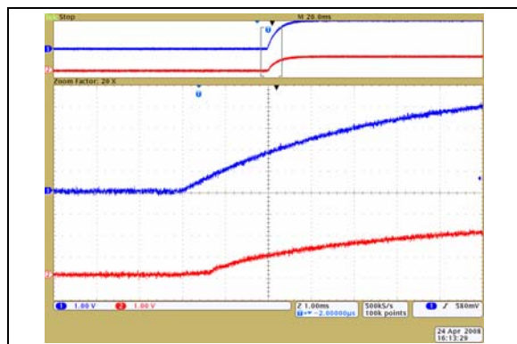
FIGURE 2-36: 50 k \Omega – Power-Up Wiper Response Time (1 \mu\text{s}/\text{Div} ).
