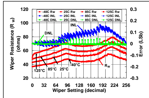
FIGURE 2-41: 100 kΩ Rheo Mode – R_W ( \Omega ), INL (LSb), DNL (LSb) vs. Wiper Setting and Ambient Temperature ( V_{DD} = 5.5\text{V} ).
