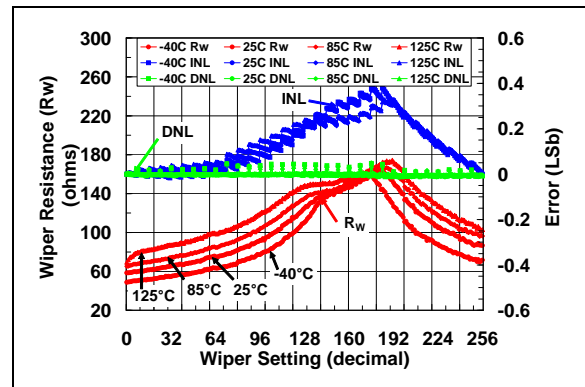
FIGURE 2-42: 100 kΩ Rheo Mode – R_W ( \Omega ), INL (LSb), DNL (LSb) vs. Wiper Setting and Ambient Temperature ( V_{DD} = 3.0\text{V} ).
