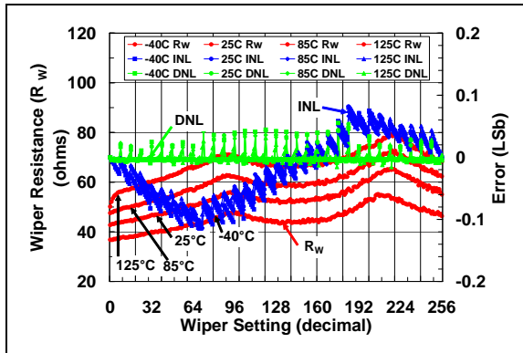
FIGURE 2-39: 100 kΩ Pot Mode – R_W ( \Omega ), INL (LSb), DNL (LSb) vs. Wiper Setting and Ambient Temperature ( V_{DD} = 5.5\text{V} ).
