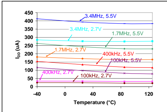
FIGURE 2-1: Device Current ( I_{DD} ) vs. f_{\text{SCL}} Frequency ( f_{\text{SCL}} ) and Ambient Temperature ( V_{DD} = 2.7\text{V} and 5.5\text{V} ).
