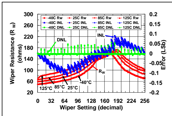
FIGURE 2-40: 100 kΩ Pot Mode – R_W ( \Omega ), INL (LSb), DNL (LSb) vs. Wiper Setting and Ambient Temperature ( V_{DD} = 3.0\text{V} ).
