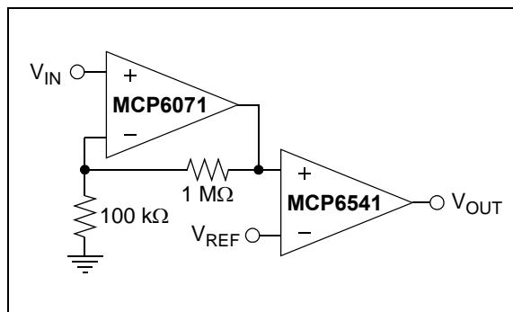
FIGURE 4-9: Precision, Non-inverting Comparator.
