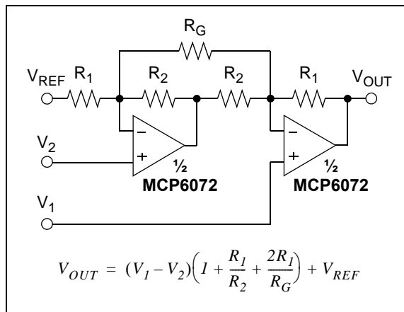
FIGURE 4-8: Two Op Amp Instrumentation Amplifier.
