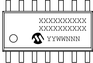
14-Lead SOIC (150 mil) (MCP6549)
