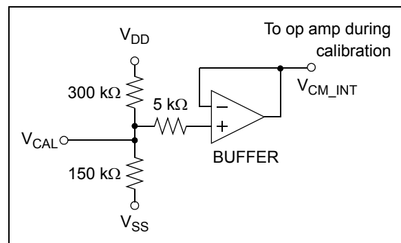
FIGURE 4-1: Common-Mode Reference's Input Circuitry.
