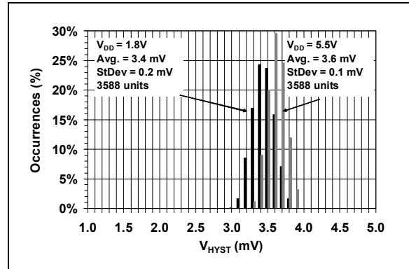
FIGURE 2-4: Input Hysteresis Voltage.
