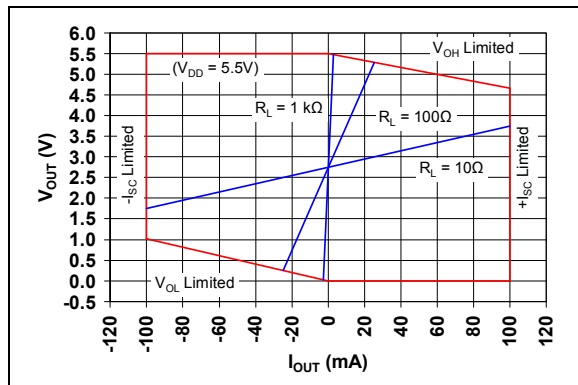
FIGURE 4-4: Output Current.
