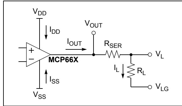
FIGURE 4-5: Diagram for Power Calculations.
