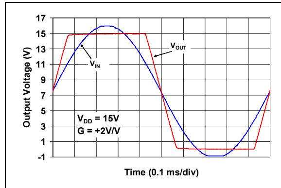
FIGURE 2-36: The MCP6H01/2 Shows No Phase Reversal.
