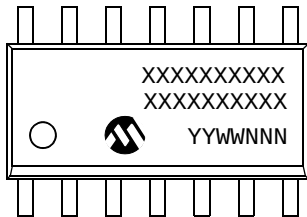
14-Lead SOIC (150 mil) (MCP6L74)
