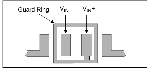
FIGURE 4-4: Example Guard Ring Layout.
