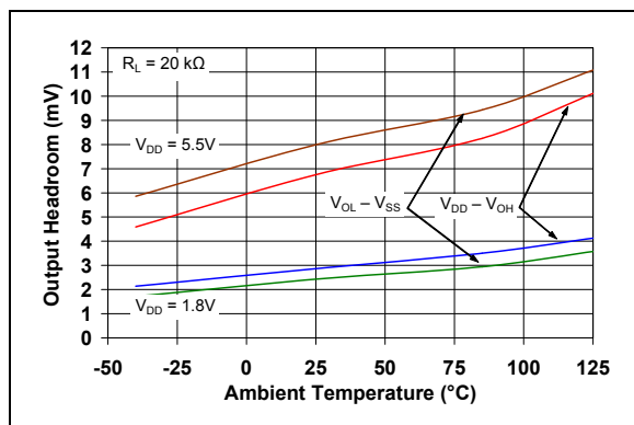
FIGURE 2-20: Output Voltage Headroom vs. Ambient Temperature.
