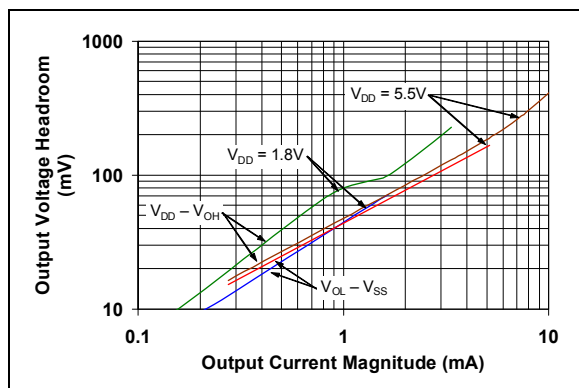
FIGURE 2-19: Output Voltage Headroom vs. Output Current.
