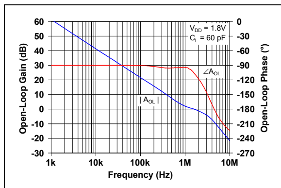
FIGURE 2-26: Open-Loop Gain vs. Frequency with V_{DD} = 1.8\text{V} .
