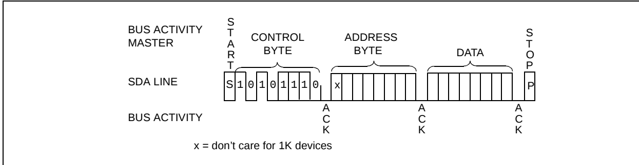
查询MCP79411供应商 FIGURE 5-3: EE BYTE WRITE
