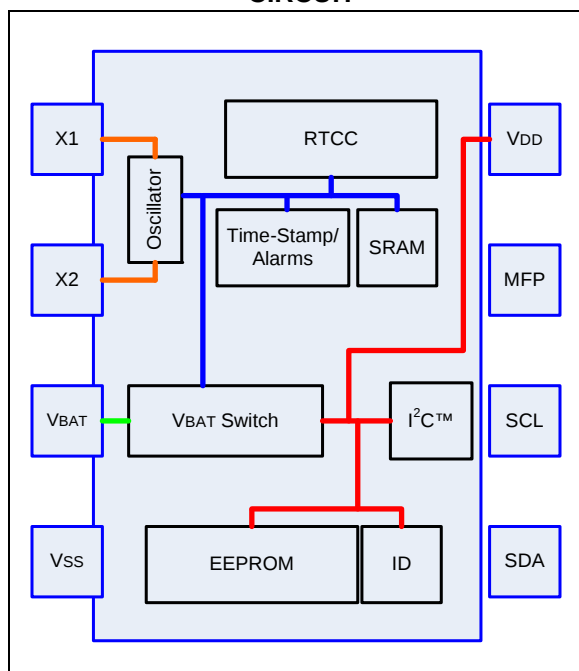
FIGURE 1-1: TYPICAL OPERATING CIRCUIT
