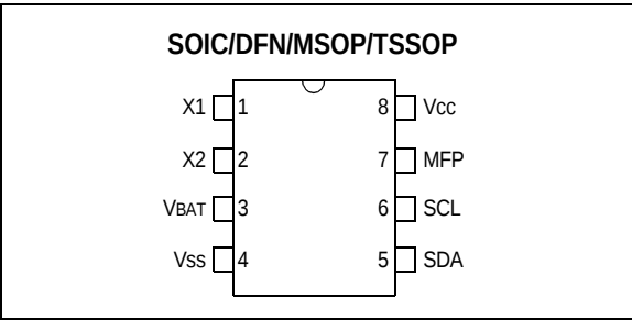
FIGURE 2-1: DEVICE PINOUTS
