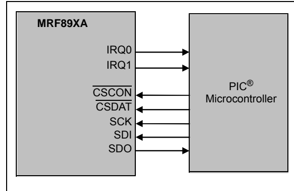
FIGURE 3-32: HOST MCU CONNECTIONS IN PACKET MODE
